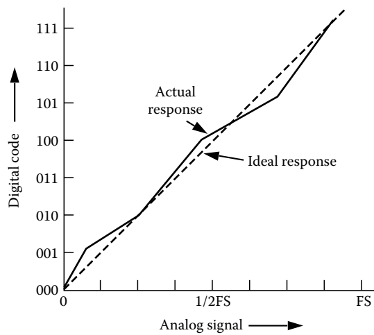
FIGURE 5.5 Monotonic nonlinearity.
