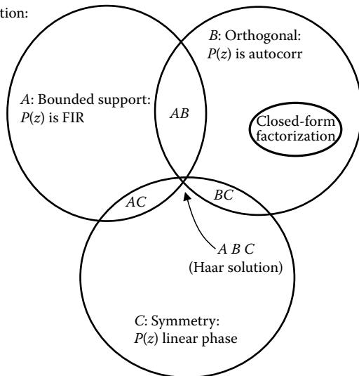
FIGURE 35.6 Two-channel perfect reconstruction filter banks. The Venn diagram illustrates which competing constraints can be simultaneously satisfied. The sets A , B , and C contain FIR, orthogonal, and linear phase solutions, respectively. Solutions in the intersection A \cap B are examined in [11,14,23,24], those in the intersection A \cap C are detailed in [12,13,15,17,25], and solutions in B \cap C are constructed in [18]. The intersection A \cap B \cap C contains only trivial solutions.
