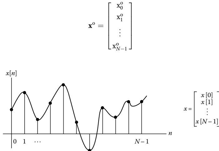
FIGURE 12.8 Representation of a random sequence as a random vector. (From Therrien, C.W., Discrete Random Signals and Statistical Signal Processing , Prentice Hall, Inc., Upper Saddle River, NJ, 1992. With permission.)
