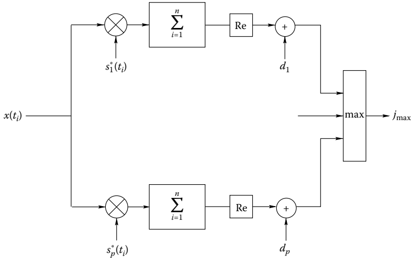
FIGURE 13.5 The ML classifier for classifying presence of one of p signals s_j(t_i) \stackrel{\text{def}}{=} s_j \underline{b}_j(t_i) , j = 1, \dots, p , under additive Gaussian white noise. d_j = -\frac{1}{2} |s_j|^2 \|\underline{b}_j\|^2 and j_{\max} is index of correlator output which is maximum. For nonwhite noise, a prewhitening transformation must be performed on x(t_i) and the \underline{b}_j(t_i) s prior to implementation of ML classifier.
