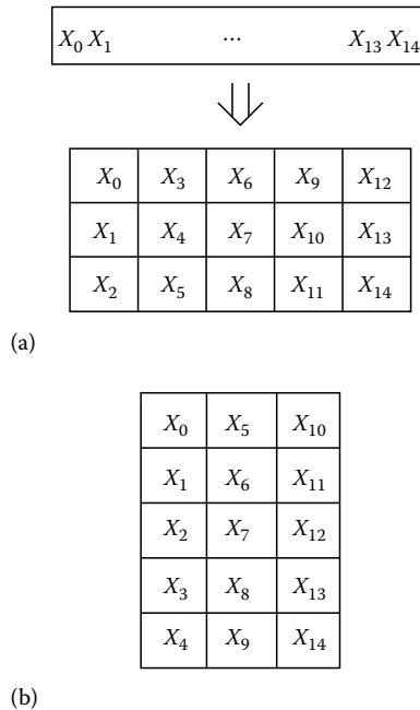
FIGURE 7.2 Cooley–Tukey mapping: (a) N_1 = 3 , N_2 = 5 and (b) N_1 = 5 , N_2 = 3 .
