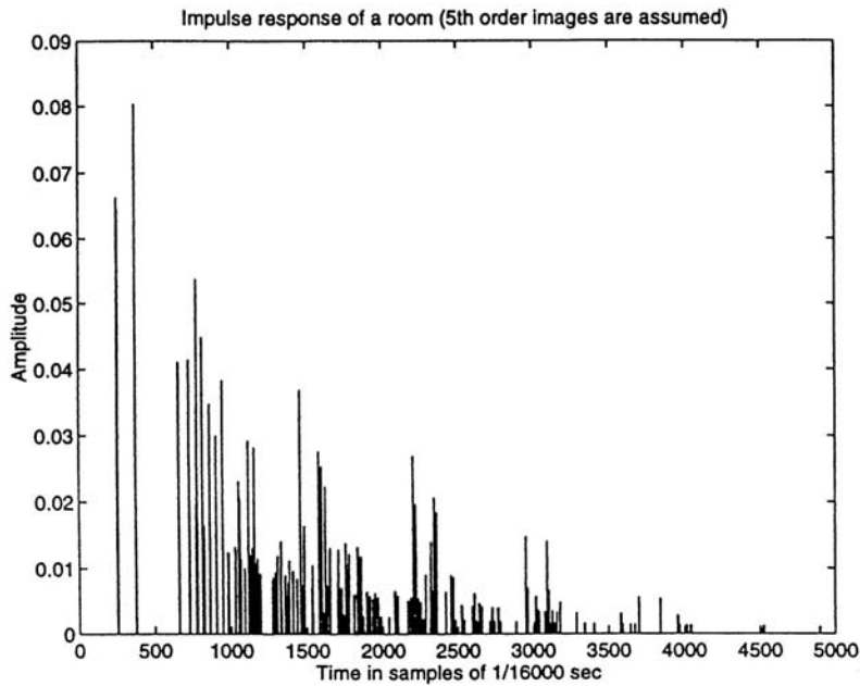
FIGURE 32.9 Impulse response of a room (images up to fifth order are used).
