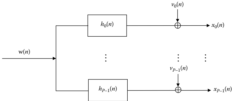
FIGURE 17.9 Multichannel stationary equivalent model of a scalar CS process.
