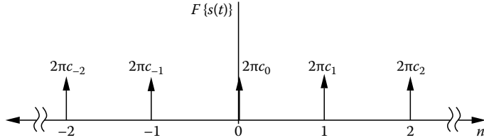
FIGURE 1.8 Spectrum of the Fourier representation of a periodic signal.
