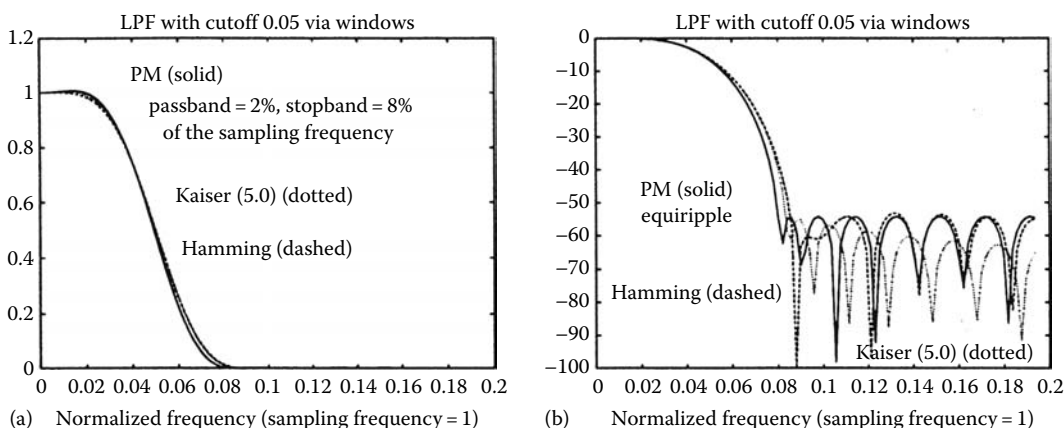
FIGURE 11.18 Comparison of window designs with optimal Chebyshev (PM) designs. The window length is N = 49 : (a) frequency response of designed filter using linear scale and (b) frequency response of designed filter using log (decibel) scale.
