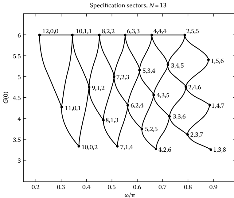
FIGURE 11.34 Specification sectors in the \omega_o – G(0) plane for length 13 filters in region I. The vertices are points at which K+L+M+1=13 . The three integers by each vertex are the flatness parameters (K, L, M) .
