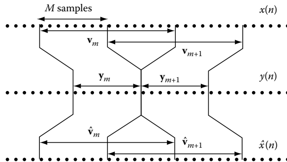
FIGURE 38.2 Illustration of an LT with N=2 applied to signal x(n) , yielding transform domain signal y(n) . The input L -tuple as vector \mathbf{v}_m is obtained by a sliding window advancing M samples, generating \mathbf{y}_m . This sliding is also valid for the synthesis side.
