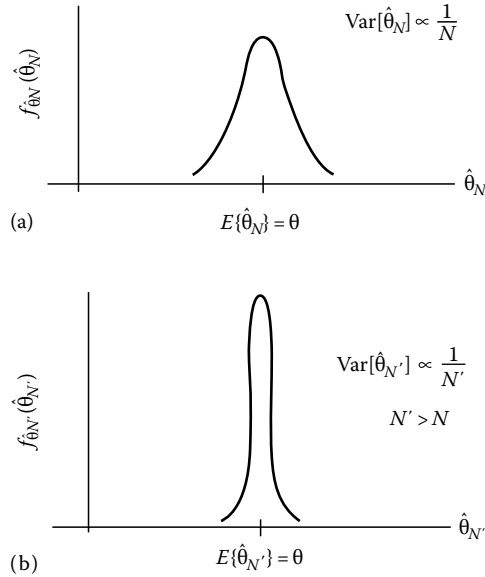
FIGURE 12.11 Density function for an unbiased estimate whose variance decreases with N : (a) density function of the estimate \hat{\theta}_N and (b) density function of the estimate \hat{\theta}_{N'} with N' > N . (From Therrien, C.W., Discrete Random Signals and Statistical Signal Processing , Prentice Hall, Inc., Upper Saddle River, NJ, 1992. With permission.)
