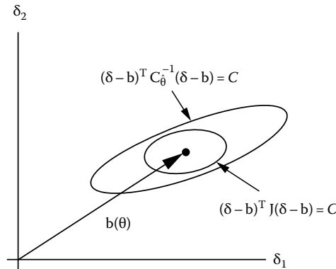
FIGURE 12.12 Concentration ellipses for the deviation of the estimate of a vector parameter; geometric interpretation of the Cramér–Rao bound. (From Therrien, C.W., Discrete Random Signals and Statistical Signal Processing , Prentice Hall, Inc., Upper Saddle River, NJ, 1992. With permission.)
