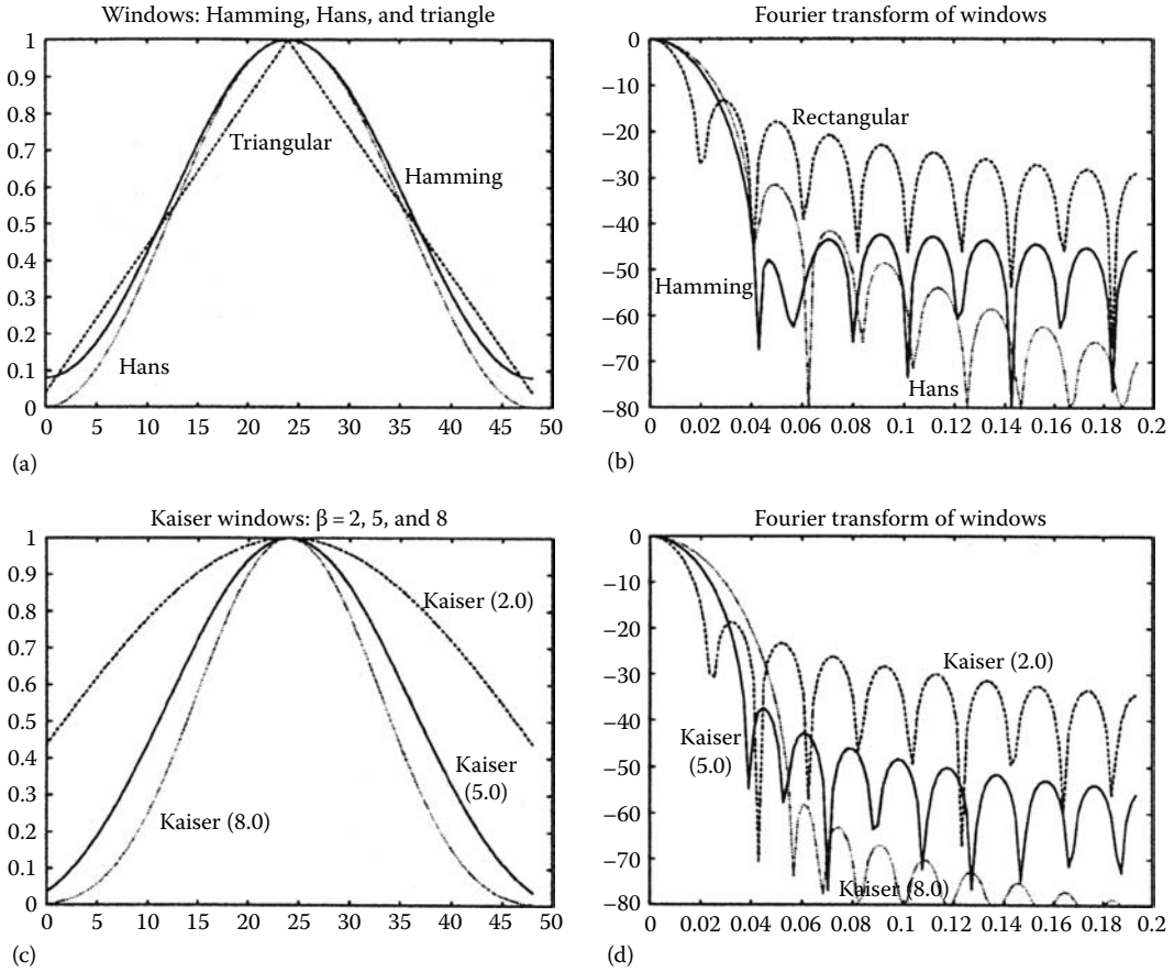
FIGURE 11.5 Common windows and their Fourier transforms. The window length is N=49 . (a) Index (a), (b) normalized frequency (sampling frequency=1), (c) Index (a), and (d) normalized frequency (sampling frequency=1).
