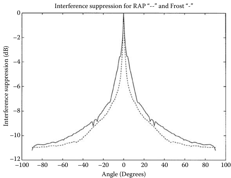
FIGURE 30.12 Interference suppression.
