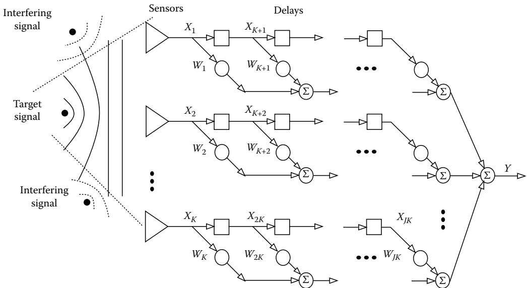
FIGURE 30.4 Broadband array.
