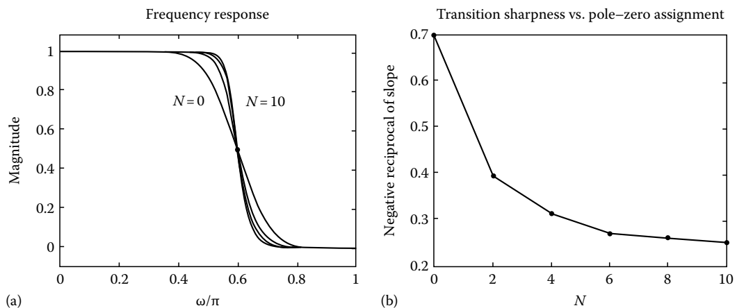
FIGURE 11.22 The filters for which the cutoff frequency is \omega_c = 0.6\pi , and for which the sum of the number of poles and the number of zeros is 20. N denotes the number of poles.
