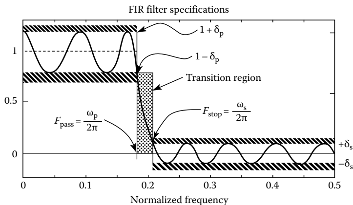
FIGURE 11.2 Design template for a lowpass filter.
