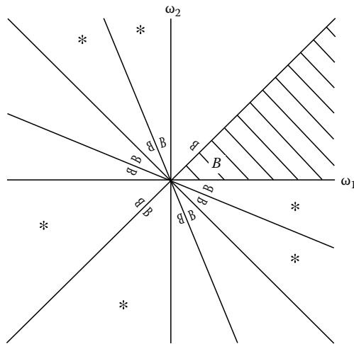
FIGURE 12.6 Regions of symmetry for the bispectrum of a real-valued signal. (From Therrien, C.W., Discrete Random Signals and Statistical Signal Processing , Prentice Hall, Inc., Upper Saddle River, NJ, 1992. With permission.)
