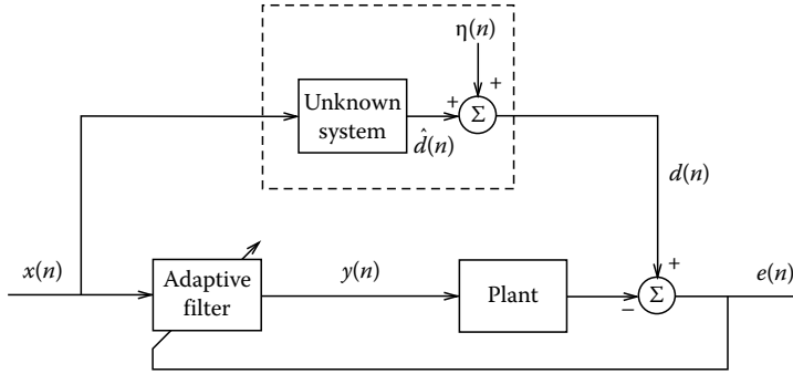
FIGURE 18.7 Feedforward control.
