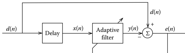
FIGURE 18.6 Linear prediction.
