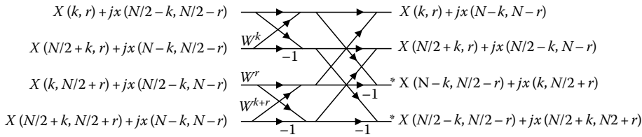
FIGURE 7.14 General VR2 butterfly.
