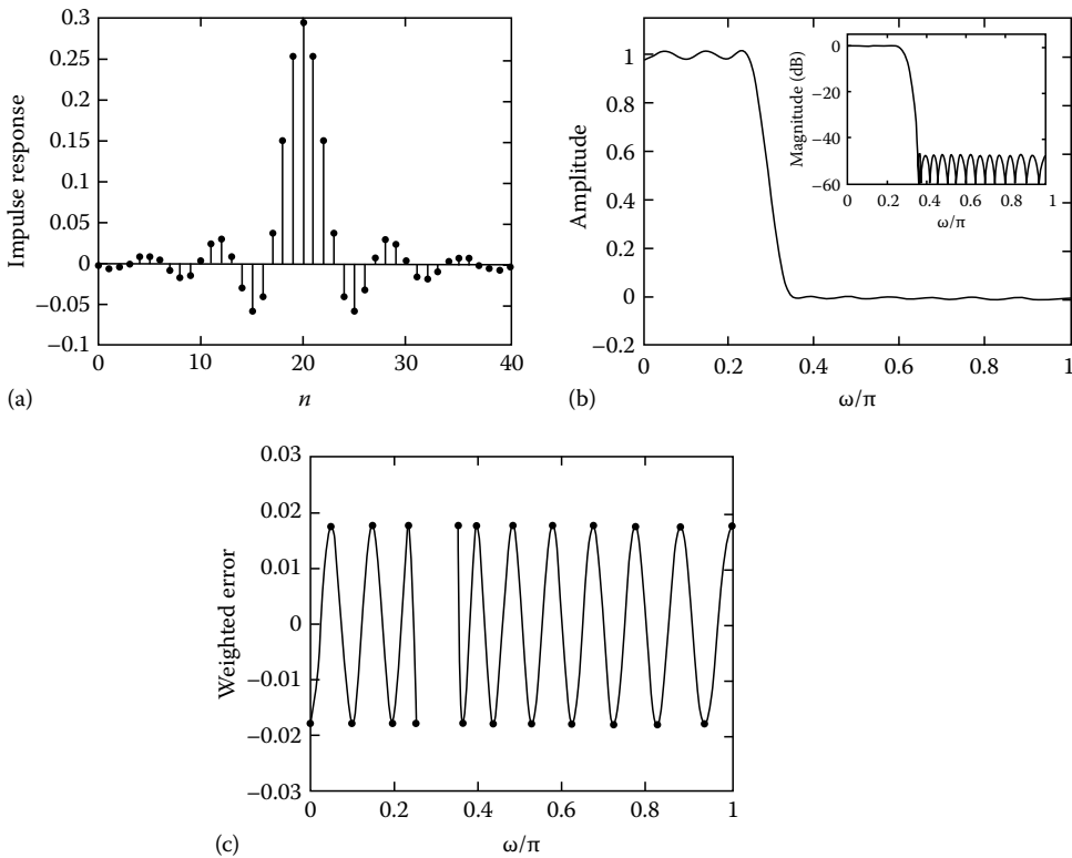
FIGURE 11.12 Equiripple lowpass filter obtained via the PM algorithm: N = 41 , \omega_p = 0.25\pi , \omega_s = 0.35\pi , and \delta_p/\delta_s = 4 .
